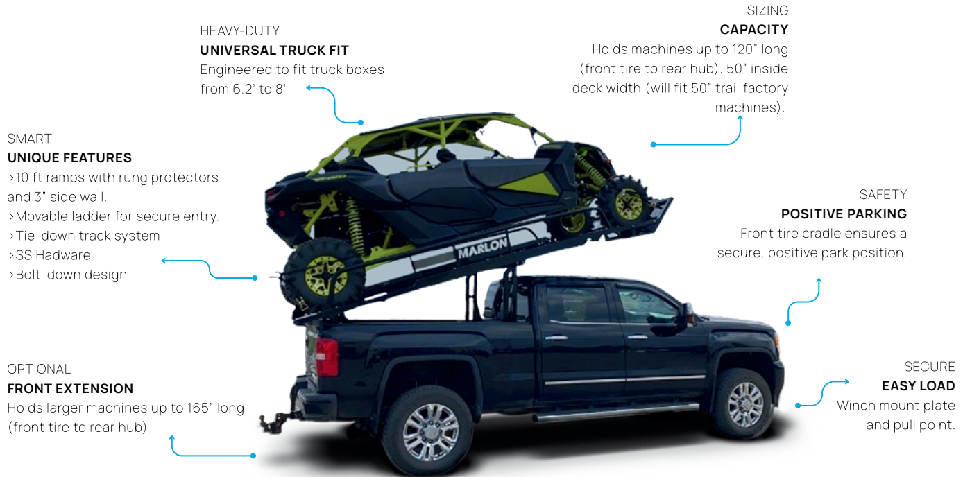
IMAGE SHOWS DECK WITH OPTIONAL FRONT EXTENSION INSTALLED
